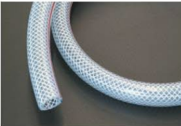
Blow-by hose Part Number: 31D003 Size: Inner Diameter 15φ, Outer Diameter 22φ Suitable for: L-shaped, 2TG, 18RG Price : ¥1,500/1m (Updated 2025.07.10)
