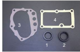
71C, 71B Packing and Seals (Updated 2025.07.20) 1.Front oil seal ¥470 2.Rear oil seal ¥430 3.Front cover gasket ¥1,010 4.71C Shift housing gasket (R32 Type M ¥480 Silvia ¥840)
