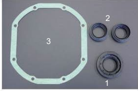
R200 Diff Parts (Updated 2025.4.9) 1.Pinion oil seal ¥980 2.Side oil seal ¥430/1pc 3.Diffcover gasket ¥2,440
