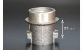
A12 Clutch sleeve (27mm) (Updated 2025.04.09) ¥1,930 *Compatible with A12 standard product A14.A15 with chromium lightweight flywheel Needs to be replaced when fitted.
