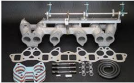
1002-PW (Pyroline gauge type) L-type 6-cylinder vehicle (for 50φ carburetor)
